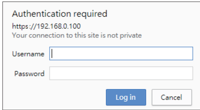
Figure 5-4: Login Screen
